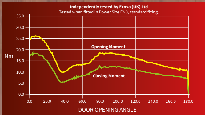
Power curve
